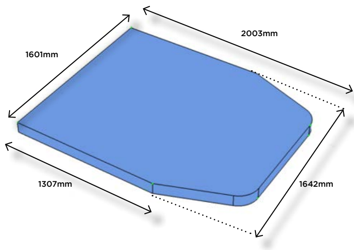
AFT CABIN
