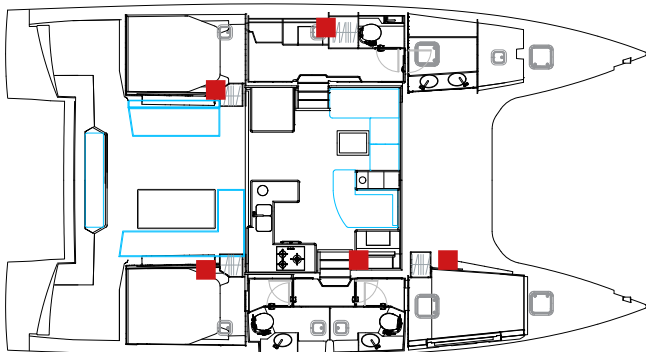
3 cabin version
