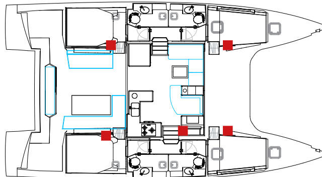
4 cabin version
